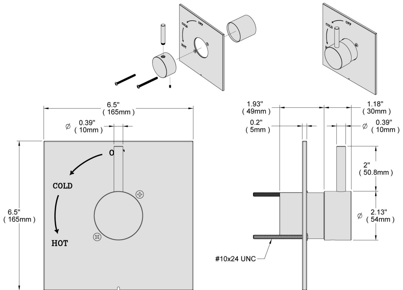
Product Diagram
